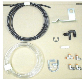
Installation Kit P/N 21999-0316
